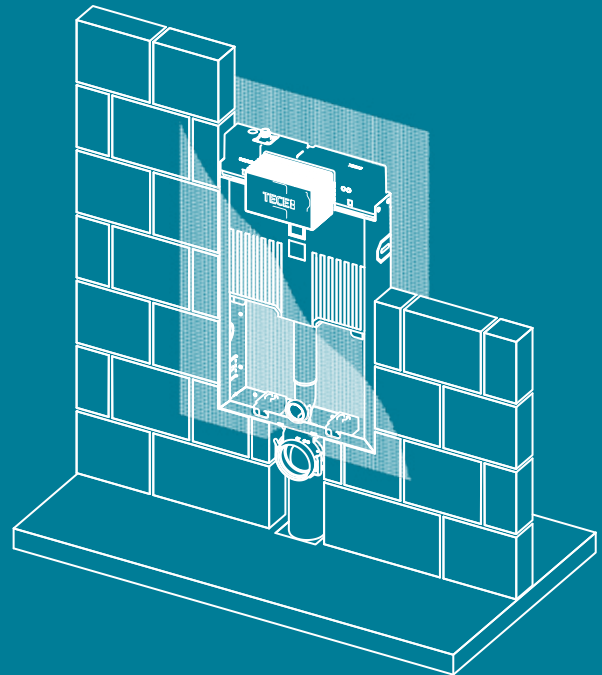
Installation in a masonry pre-wall
