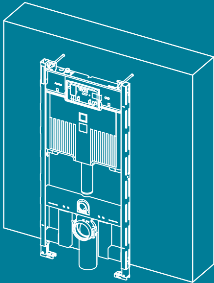
Individual module installation in front of a solid structural shell wall
