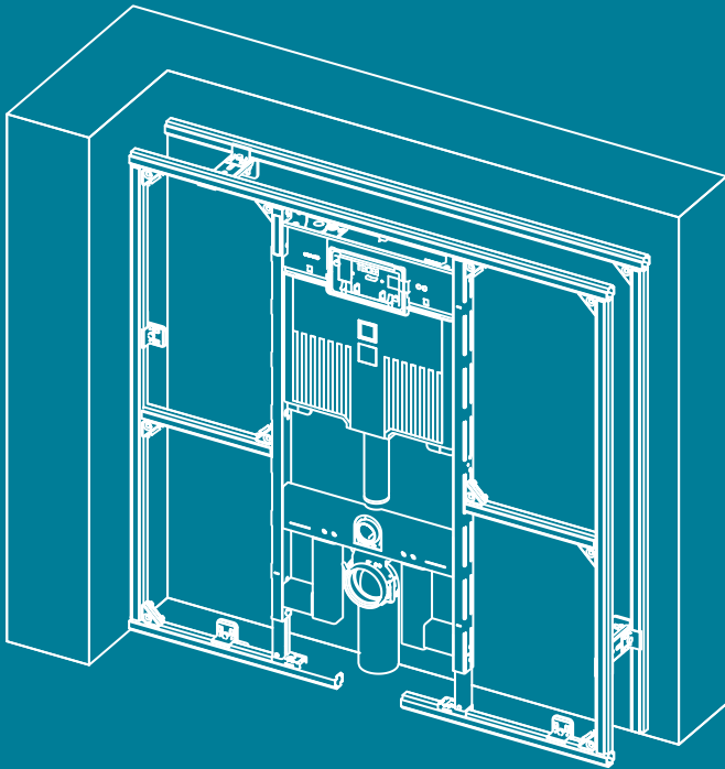
Installation in a TECEprofil pre-wall
