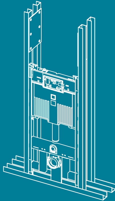
Installation in metal profiles and wooden stud walls
